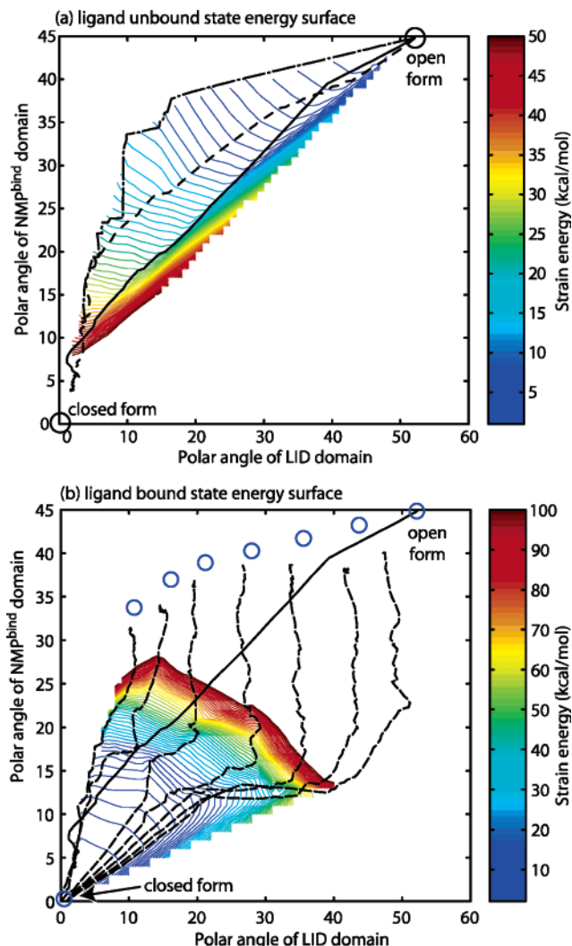
Figure 5. Energy surface with reaction coordinates polar rotation angle of LID and NMP bind domain. The origin of polar axes ( 0^\circ, 0^\circ ) is the closed form. (a) The energy surface of the ligand-unbound state. The nonlinear paths from open form by iteration with 3 modes (solid line), with 2 modes (broken line), and with 1 mode (dash-dot line) are projected in this angular coordinate space. The interpolated strain energy surface of the open state is superimposed as contour lines. (b) The energy surface of the ligand-bound state. Conformational change paths from the closed form toward different target structures are projected in the angular coordinate space (broken lines). Targets used to generate these paths were the 0th, 10th, ..., and 60th structures along the path from the open form that were generated using 1 mode, shown in (O). These paths are used to obtain the energy surface of the ligand-bound state, which are shown as contour lines. The nonlinear path from the open form toward the closed form by iteration with 3 modes is shown by a solid line.
