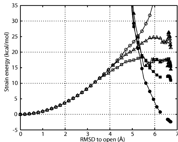
Figure 7. Energy surface with cracking effects. Calculations of energy profiles from the nonlinear elastic model without cracking are marked (O), with cracking and surface tension \sigma = 1 are ( \Delta ), and with cracking for \sigma = 0.5 kcal/mol are ( \square ). Energies of the ligand-unbound state are shown by open markers, and the ligand bound state are shown by filled markers. Free energy change of \Delta G_{\text{react}} = -3 kcal/mol is employed in this figure as a representative. The cracking effect lowers the energy barrier. The energy surface of the ligand bound states with low surface tension has higher energy than one without cracking, since some residues are partially unfolded. Actual conformational change would involve a refolding process, i.e., shift from the energy profile with cracking to the energy profile without cracking.
