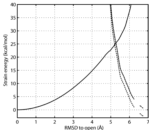
Figure 6. Superposition of energy profiles of the ligand-unbound and bound states along a representative conformational change path, which is obtained from the 2-dimensional energy surfaces (Figure 5). The energy profile of the open state is indicated by a solid line, the closed form with free energy change \Delta G_{\text{react}} = 0 kcal/mol by a broken line, and \Delta G_{\text{react}} = -3 kcal/mol by a dotted line.
