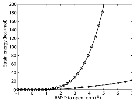
Figure 3. Comparison between energy surface, explicitly calculated, for the structures linearly deformed along mode 1, the lowest frequency mode, which is most relevant to the conformational change (○), and the energy surface modeled from the frequency of mode 1 at the initial state on the normal mode coordinate 1. RMSD = 5.9 Å corresponds to the projection of the final state on the normal mode coordinate 1. Explicitly calculated energy surface along mode 1 shows significant deviation from the harmonic surface.
