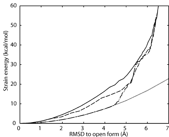
Figure 4. Energy surface along nonlinear conformational change path by iterative method. (a) Energy of structures along the path that was generated from the open form by iterative method using the highest overlap mode (dash-dot line), two highest modes (broken line), and three modes (solid line). The pure harmonic energy surface expected from the frequency of the lowest frequency mode is shown for comparison (dotted line).
