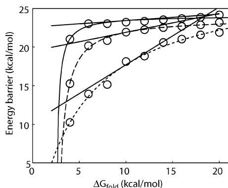
Figure 9. Transition state barrier dependence on the cracking threshold. This figure shows how the transition state barrier, \Delta G^* , depends on the protein stability, \Delta G_{\text{fold}} . A driving force of \Delta G_{\text{react}} = -3 kcal/mol is used. Three values of surface tension, \sigma = 1.5, 1, or 0.5 kcal/mol, are tested. For each \sigma = 1.5 kcal/mol (solid line), \sigma = 1 kcal/mol (broken line), and \sigma = 0.5 kcal/mol (dotted line), the data are fitted hyperbolically to \partial\Delta G^* = -4.9/(\Delta G_{\text{fold}} - 2.4) + 24 , \partial\Delta G^* = -14/(\Delta G_{\text{fold}} - 2.3) + 24 , and \partial\Delta G^* = -167/(\Delta G_{\text{fold}} + 4.9) + 28 , respectively. From the slope of the line, the slope \alpha = \partial\Delta G^*/\partial\Delta G_{\text{fold}} at \Delta G_{\text{fold}} = 10 kcal/mol is estimated as 0.084 for \sigma = 1.5 kcal/mol, 0.24 for \sigma = 1 kcal/mol, and 0.75 for \sigma = 0.5 kcal/mol. These are used for the estimations of \partial\Delta G^*/\partial[\text{urea}] in the main text.
