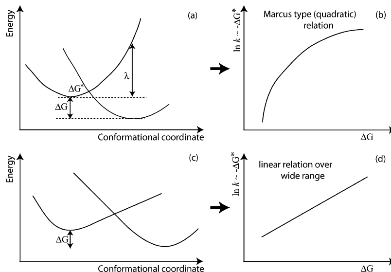
Figure 1. Schematic representation of the reaction rate dependence on the character of two energy surfaces. When the two energy surfaces are quadratic (a), the activation energy is related to the reaction free energy, \Delta G , and the reorganization energy, \lambda , by eq 2, as in the theory of electron-transfer reactions. In this case, the reaction rate depends quadratically on the driving force ( -\Delta G ) (b). When the two energy surfaces are linear (c), the rate depends on the driving force linearly (d).
