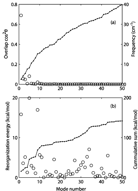
Figure 2. Estimation of the reorganization energy using simple normal-mode analysis. (a) Frequency (solid line) and degree of overlap (O) between the conformational change and each of calculated normal modes. The conformational change can be mostly described by a few low-frequency modes. (b) Contribution of each normal mode to the total reorganization energy, obtained from the linear elastic model, eq 3. Cumulative sum of contributions is shown by a solid line.
