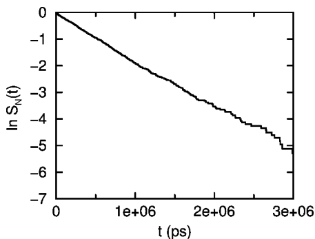
FIG. 1. The time dependence of \ln S_N(t) for the system in which no molecular interactions were included (system 1). The ligand concentration was 0.0001M .
